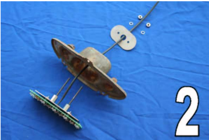
Pass the LED wire through the taillight and brackets as shown.
